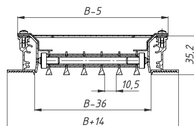
VLLS-S
