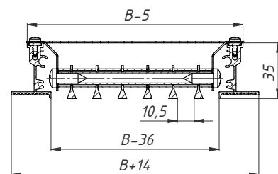
VLL-S
